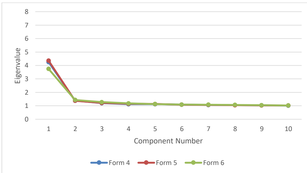
Figure 42. Dimensionality Report of Principal Component Eigenvalues, GED® Reasoning Through Language Arts, Spanish, Forms 4, 5, and 6
