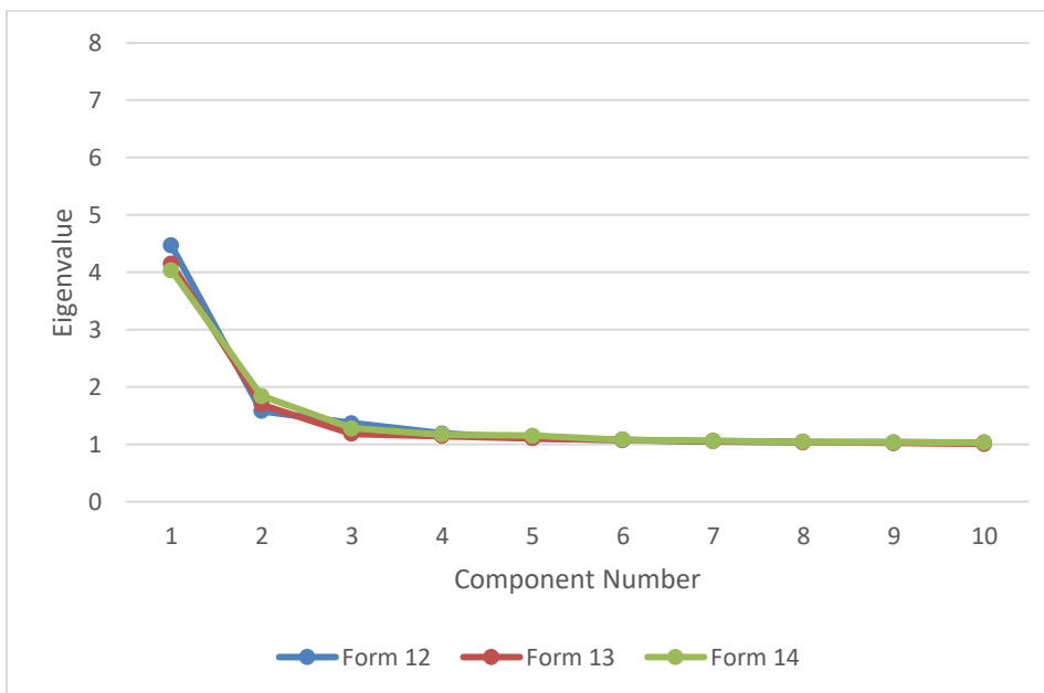
Figure 40. Dimensionality Report of Principal Component Eigenvalues, GED® Mathematical Reasoning, Spanish, Forms 12, 13, and 14
