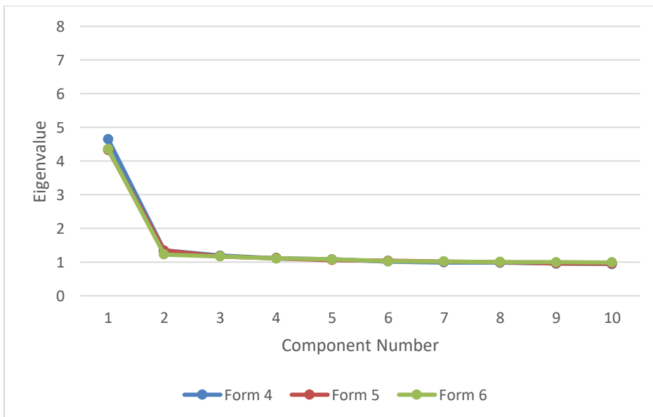
Figure 20. Dimensionality Report of Principal Component Eigenvalues, GED® Science, English, Forms 4, 5, and 6
