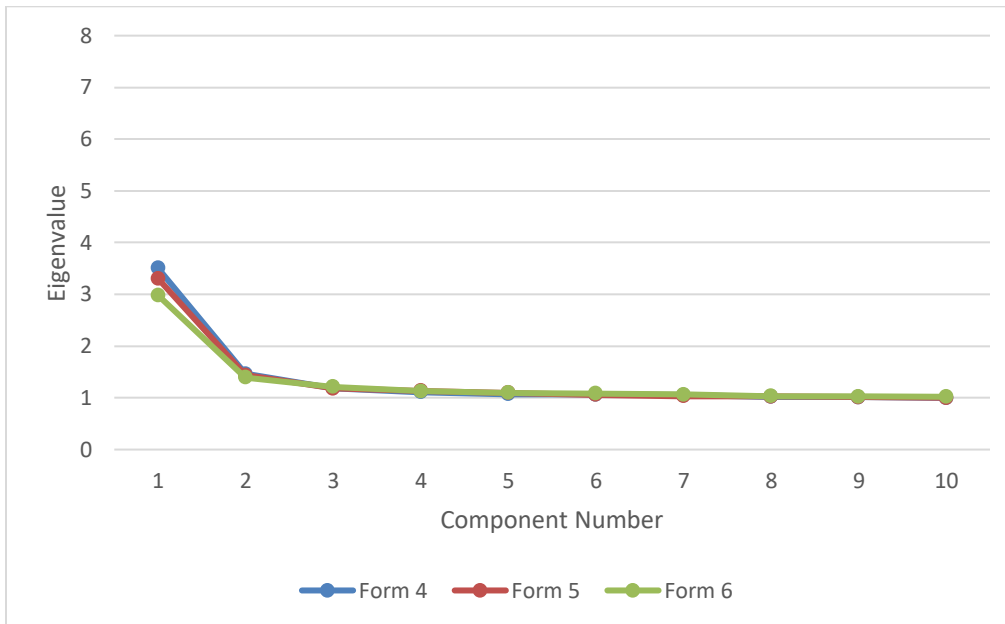
Figure 46. Dimensionality Report of Principal Component Eigenvalues, GED® Science, Spanish, Forms 4, 5, and 6
