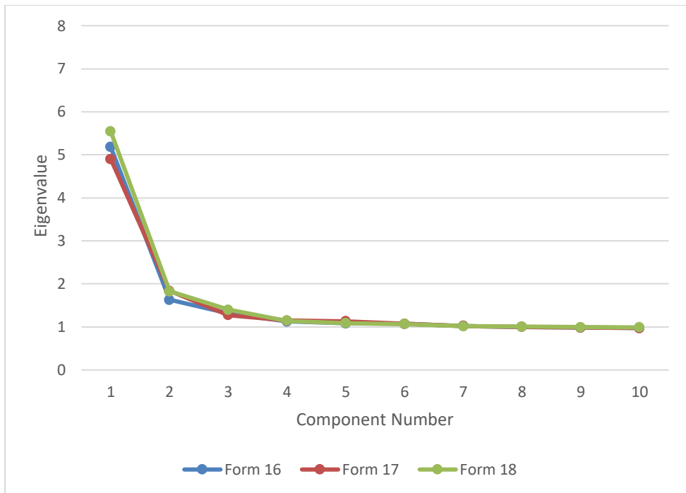
Figure 8. Dimensionality Report of Principal Component Eigenvalues, GED® Mathematical Reasoning, English, Forms 16, 17, and 18
