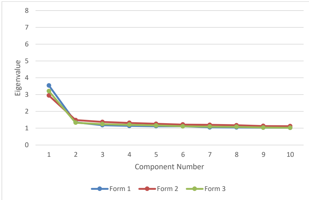
Figure 45. Dimensionality Report of Principal Component Eigenvalues, GED® Science, Spanish, Forms 1, 2, and 3
