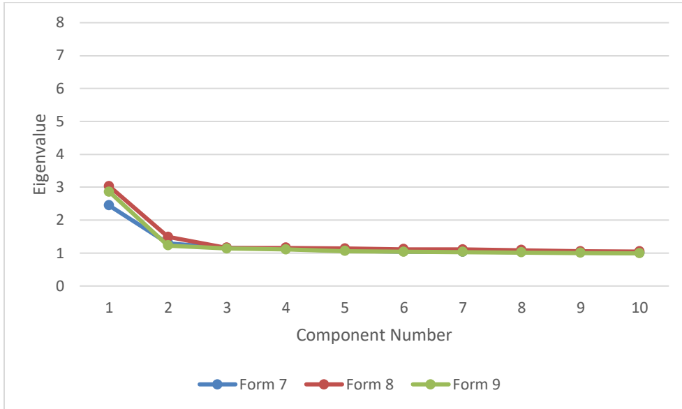
Figure 52. Dimensionality Report of Principal Component Eigenvalues, GED® Social Studies, Spanish, Forms 7, 8, and 9
