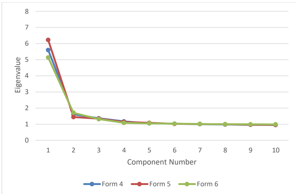
Figure 4. Dimensionality Report of Principal Component Eigenvalues, GED® Mathematical Reasoning, English, Forms 4, 5, and 6
