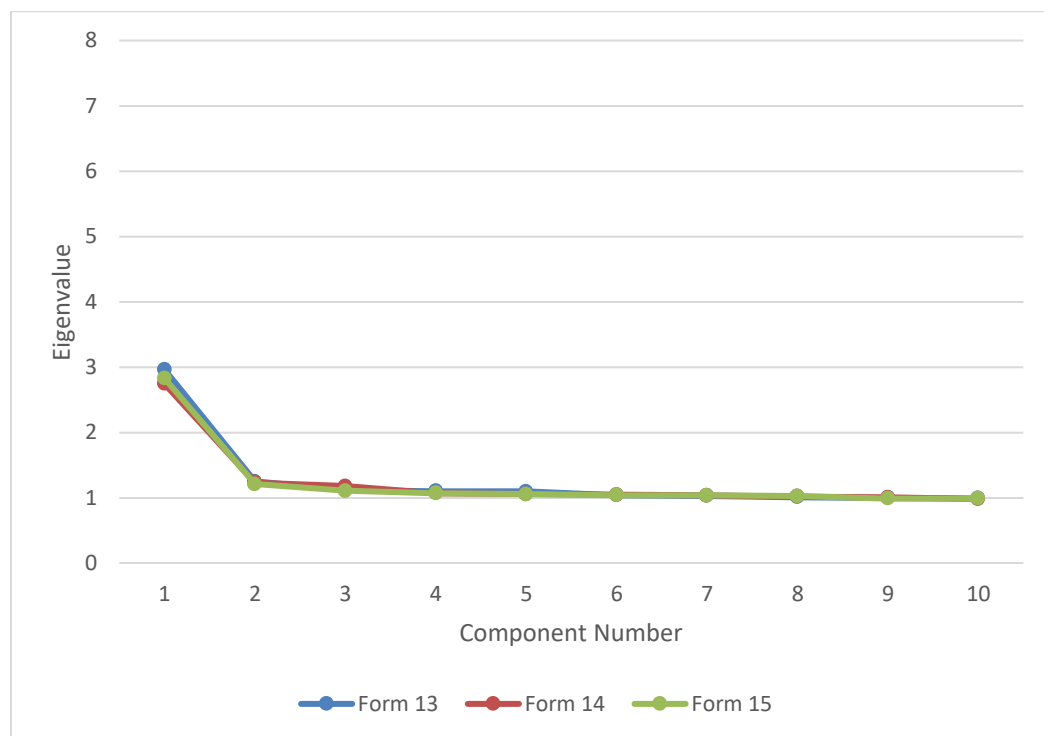
Figure 54. Dimensionality Report of Principal Component Eigenvalues, GED® Social Studies, Spanish, Forms 13, 14, and 15
