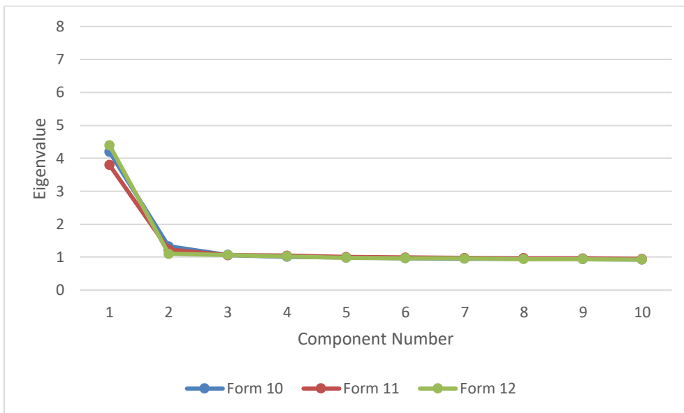
Figure 30. Dimensionality Report of Principal Component Eigenvalues, GED® Social Studies, English, Forms 10, 11, and 12
