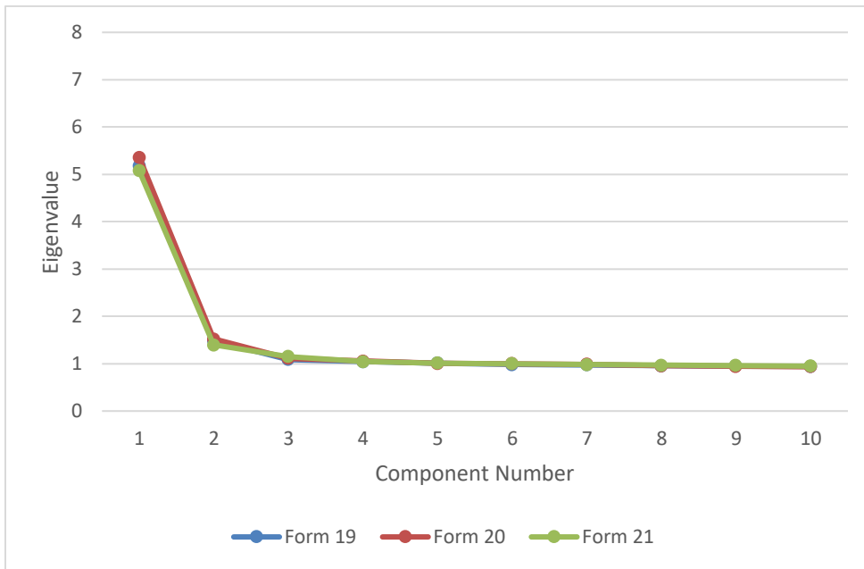
Figure 25. Dimensionality Report of Principal Component Eigenvalues, GED® Science, English, Forms 19, 20, and 21
