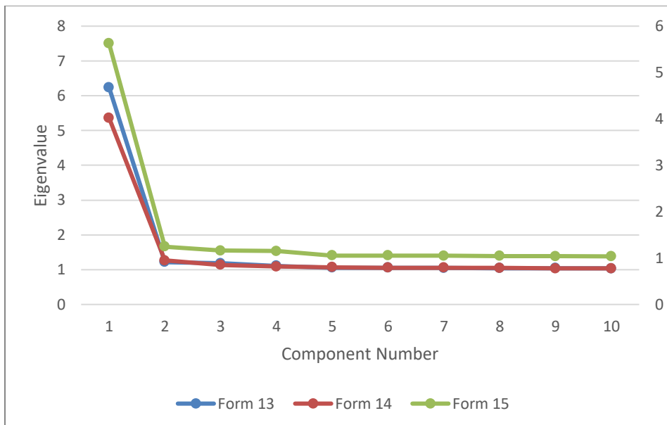
Figure 16. Dimensionality Report of Principal Component Eigenvalues, GED® Reasoning Through Language Arts, English, Forms 13, 14, and 15
