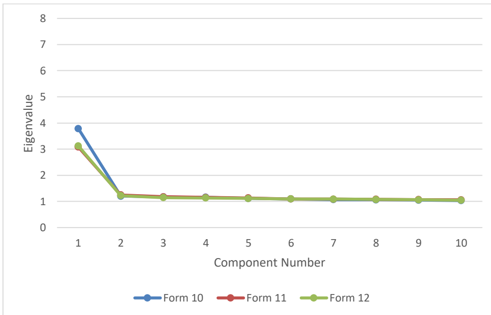
Figure 44. Dimensionality Report of Principal Component Eigenvalues, GED® Reasoning Through Language Arts, Spanish, Forms 10, 11, and 12
