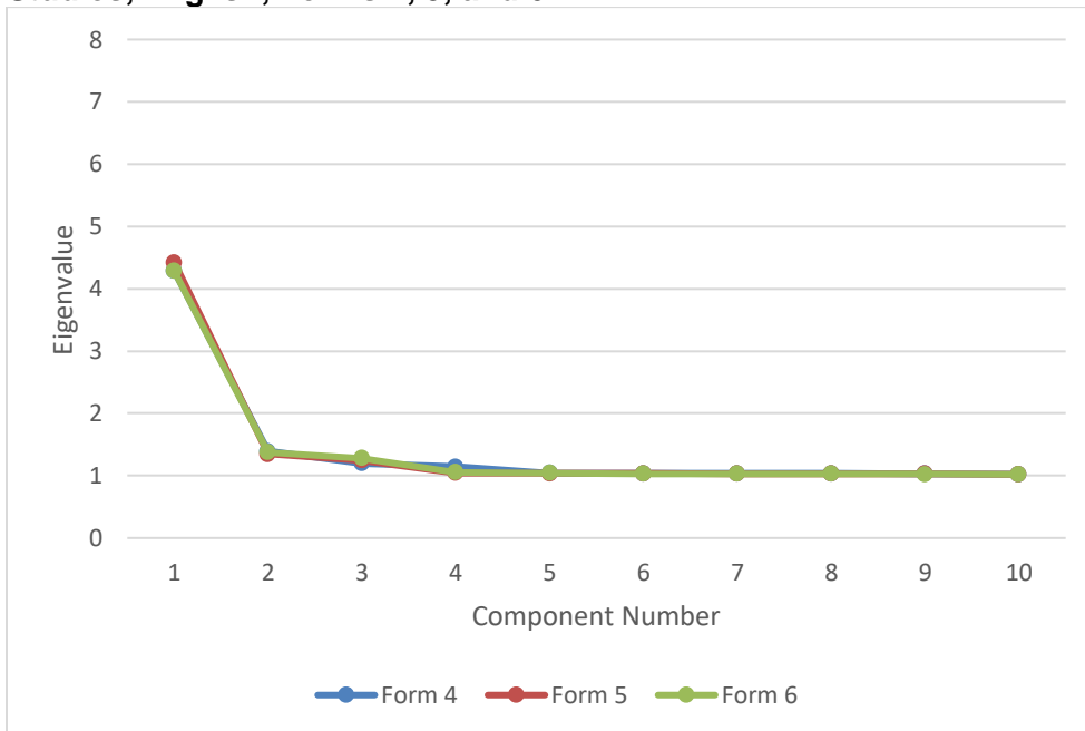
Figure 28. Dimensionality Report of Principal Component Eigenvalues, GED® Social Studies, English, Forms 4, 5, and 6
