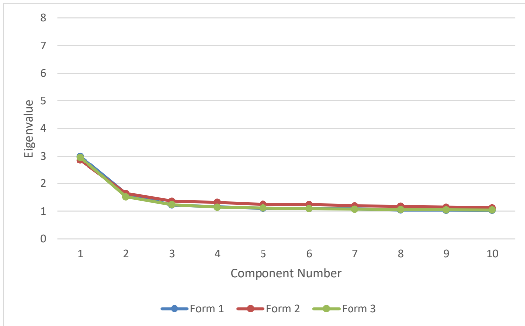
Figure 50. Dimensionality Report of Principal Component Eigenvalues, GED® Social Studies, Spanish, Forms 1, 2, and 3
