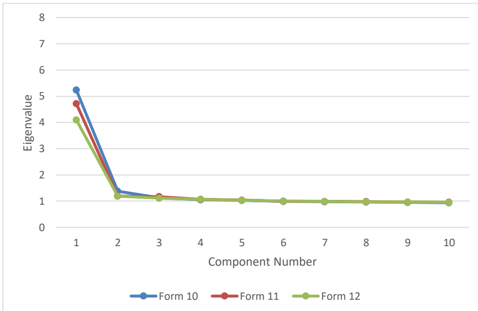
Figure 22. Dimensionality Report of Principal Component Eigenvalues, GED® Science, English, Forms 10, 11, and 12
