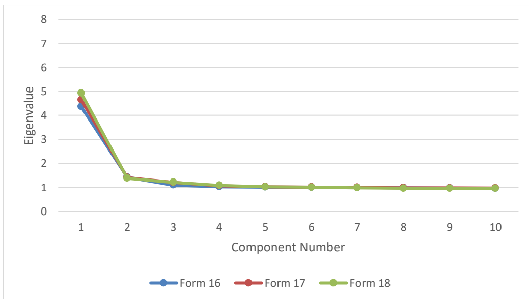
Figure 24. Dimensionality Report of Principal Component Eigenvalues, GED® Science, English, Forms 16, 17, and 18
