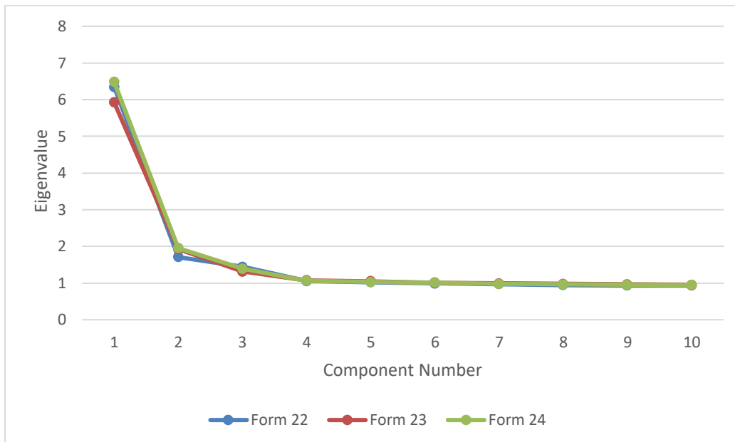
Figure 10. Dimensionality Report of Principal Component Eigenvalues, GED® Mathematical Reasoning, English, Forms 22, 23, and 24
