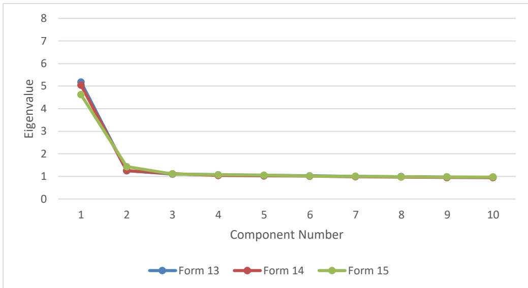
Figure 23. Dimensionality Report of Principal Component Eigenvalues, GED® Science, English, Forms 13, 14, and 15
