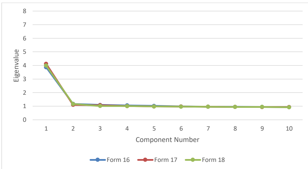
Figure 32. Dimensionality Report of Principal Component Eigenvalues, GED® Social Studies, English, Forms 16, 17, and 18
