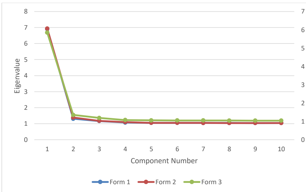
Figure 12. Dimensionality Report of Principal Component Eigenvalues, GED® Reasoning Through Language Arts, English, Forms 1, 2, and 3
