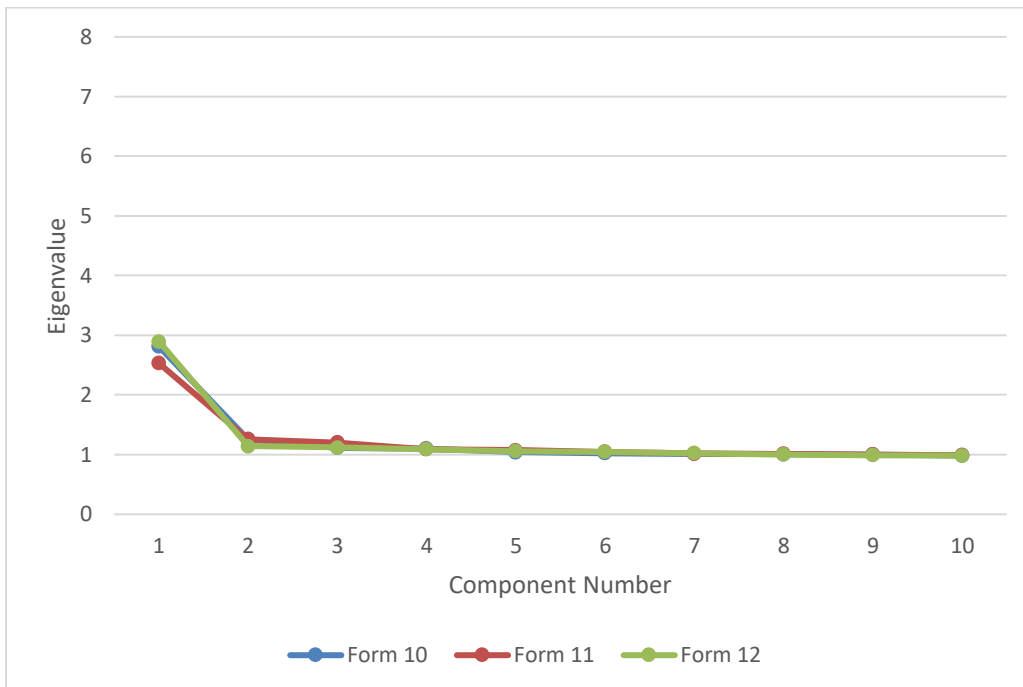
Figure 53. Dimensionality Report of Principal Component Eigenvalues, GED® Social Studies, Spanish, Forms 10, 11, and 12
