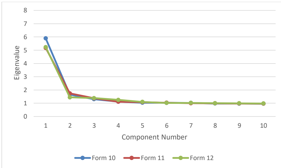
Figure 6. Dimensionality Report of Principal Component Eigenvalues, GED® Mathematical Reasoning, English, Forms 10, 11, and 12
