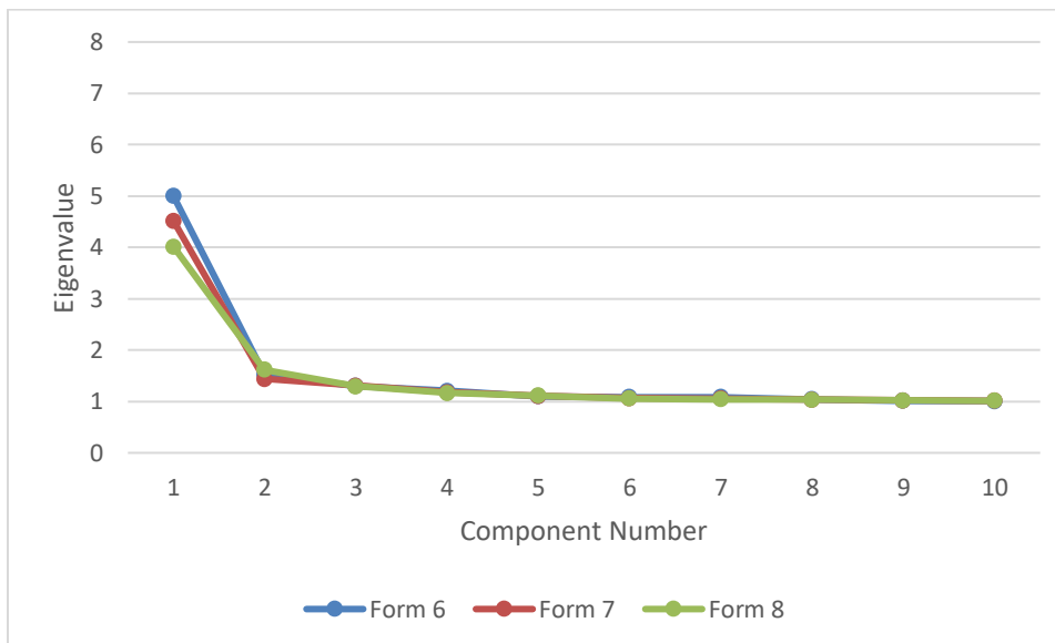
Figure 38. Dimensionality Report of Principal Component Eigenvalues, GED® Mathematical Reasoning, Spanish, Forms 6, 7, and 8
