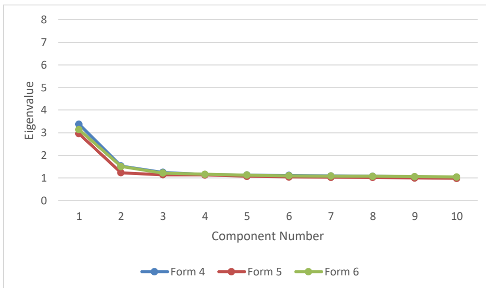
Figure 51. Dimensionality Report of Principal Component Eigenvalues, GED® Social Studies, Spanish, Forms 4, 5, and 6
