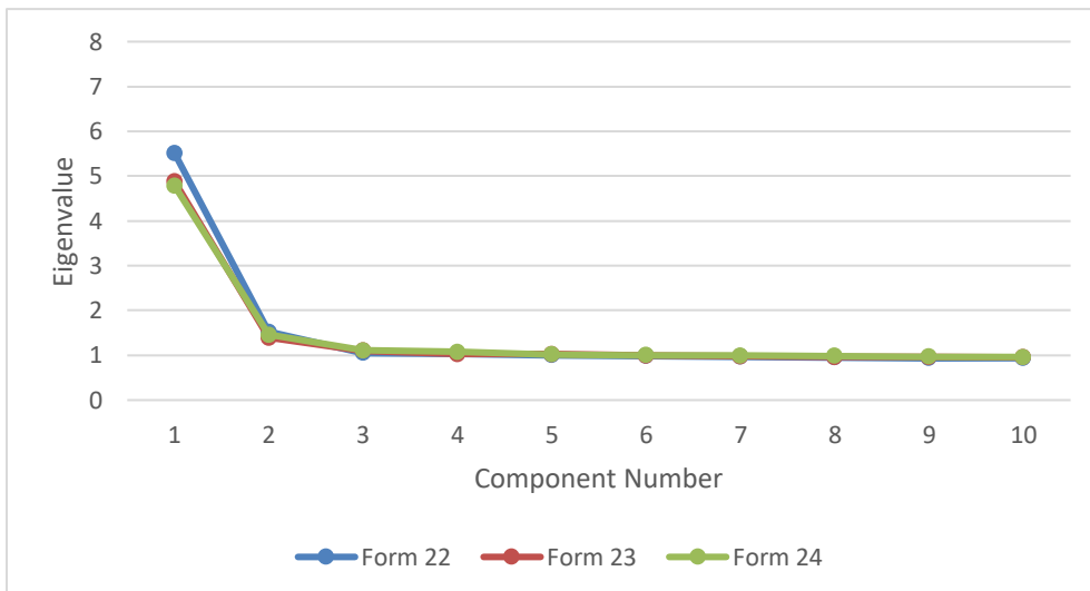
Figure 26. Dimensionality Report of Principal Component Eigenvalues, GED® Science, English, Forms 22, 23, and 24
