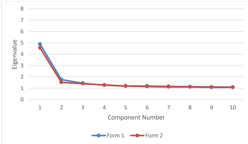
Figure 36. Dimensionality Report of Principal Component Eigenvalues, GED® Mathematical Reasoning, Spanish, Forms 1 and 2
