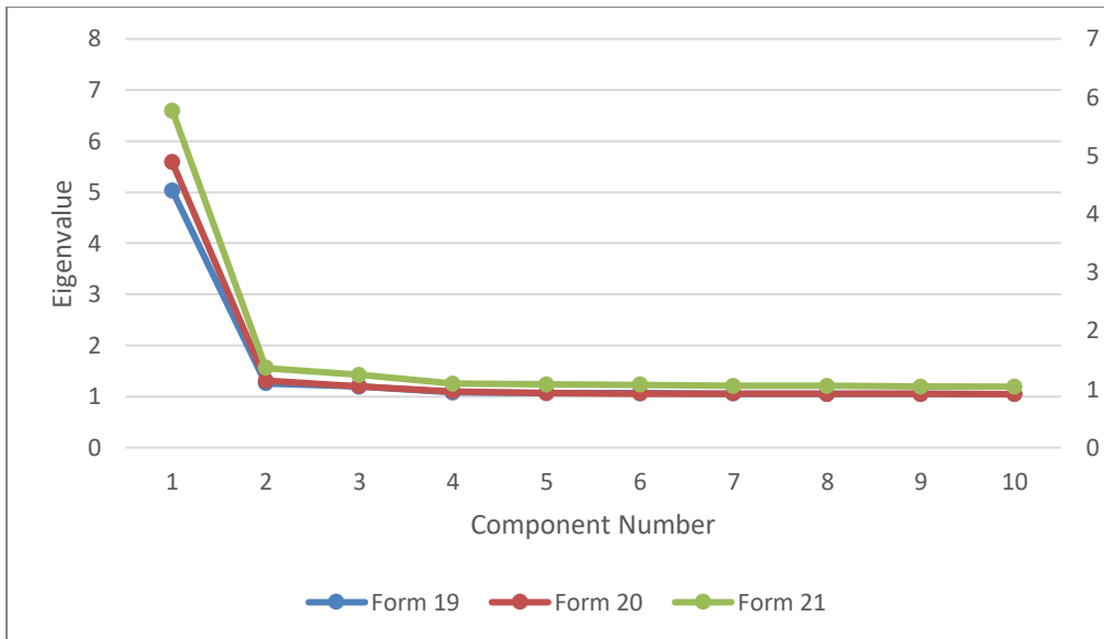
Figure 18. Dimensionality Report of Principal Component Eigenvalues, GED® Reasoning Through Language Arts, English, Forms 19, 20, and 21
